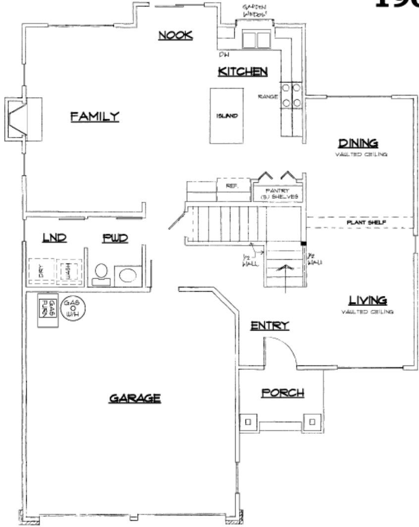
MAIN FLOOR
