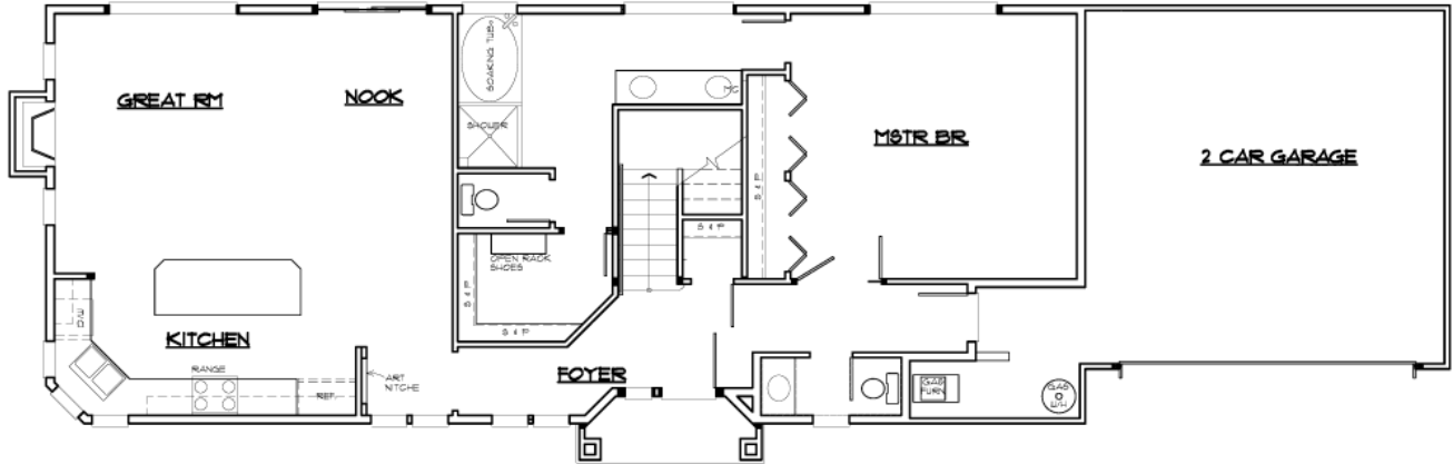
MAIN FLOOR PLAN
