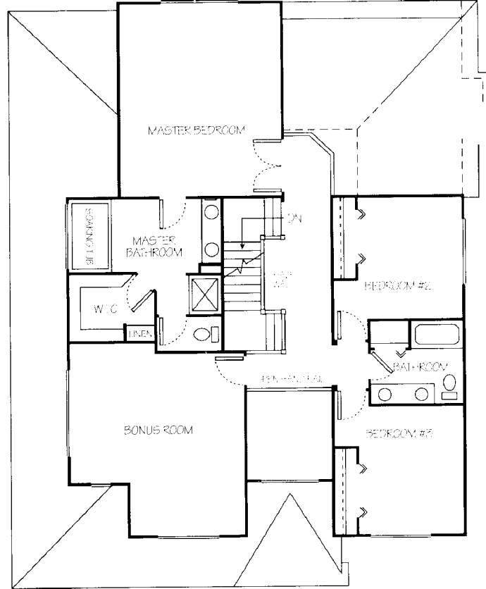
Upper Floor; Master Back
