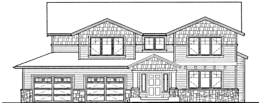
ELEVATION C
