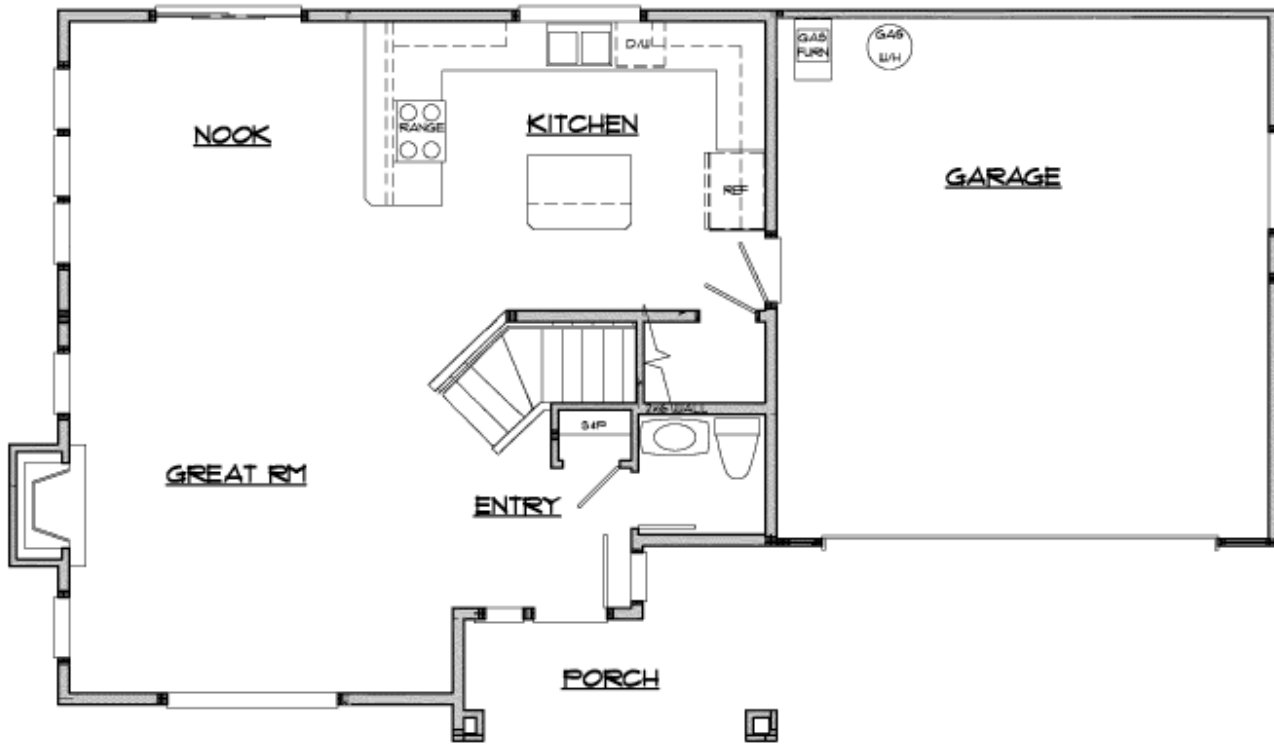
MAIN FLOOR
